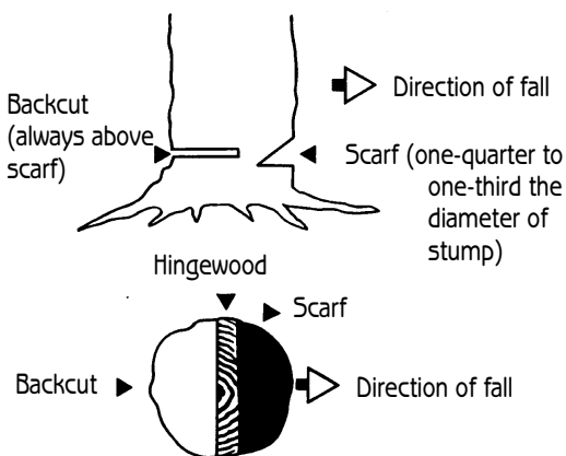
Scarf, backcut and hingewood.
